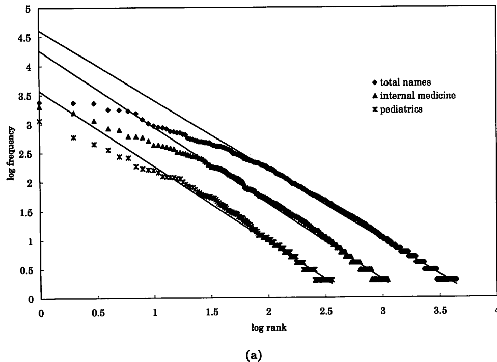
Fig. 1 Zipf plots of the freely written group. A logarithm of the frequency vs. a logarithm of the rank is plotted on the figures. The straight lines denote regression lines of data: (a) total diagnoses, internal medicine and pediatrics, and (b) Surgery, ophthalmology and dermatology.
