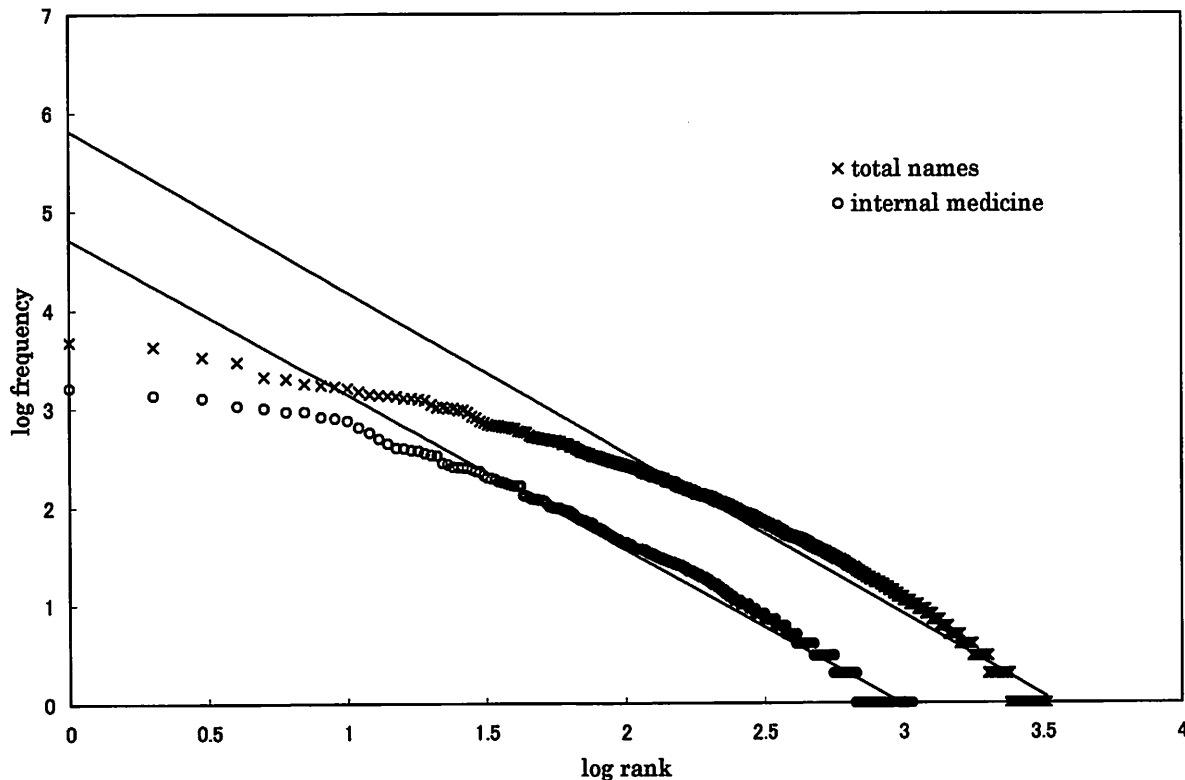
Fig. 3 Zipf plots of total diagnoses and internal medicine in the coded group. The data show large deviations from the regression lines, which are denoted by the straight line in the figure.
