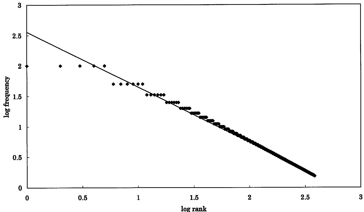
Fig. 4 Zipf plot of the union of five Zipf sets. The Zipf plot of the union of five sets, each of which follow Zipf's law and has no common diagnosis. Figure shows that this union asymptotically follows Zipf's law, but at high frequencies, data deviate from the regression line.
